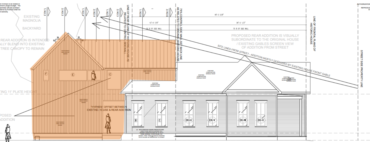
2 COMBINED NEW SOUTH SIDE YARD) ELEVATION: WITH NEW ADDITION BEHIND ORIGINAL GABLE ROOF
