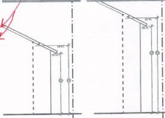
PRIMARY BUILDING 1-STORY EAVE HEIGHT RANGE
