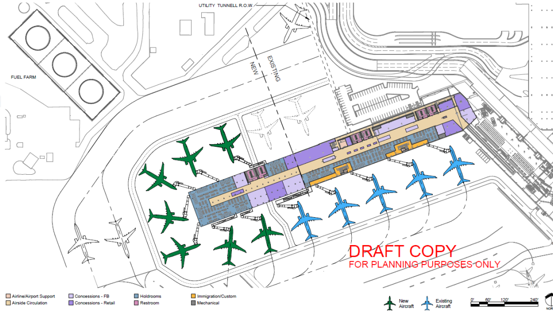
COLOR BLOCK PLAN - 02 CONCOURSE LEVEL - 7 GATE
